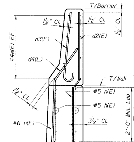
REINFORCING
