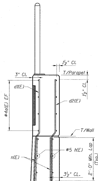
REINFORCING
