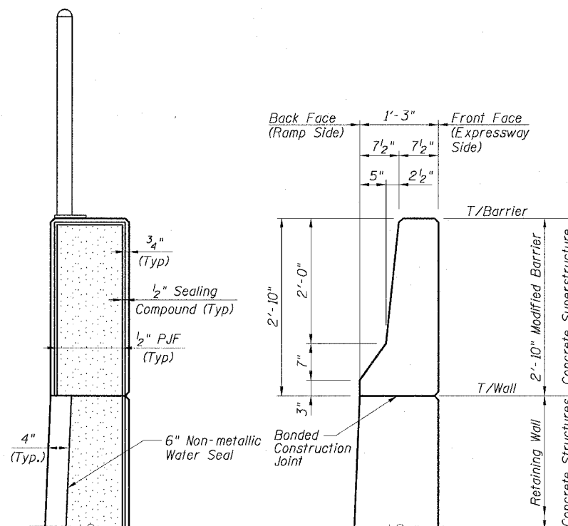
EXPANSION JOINT
