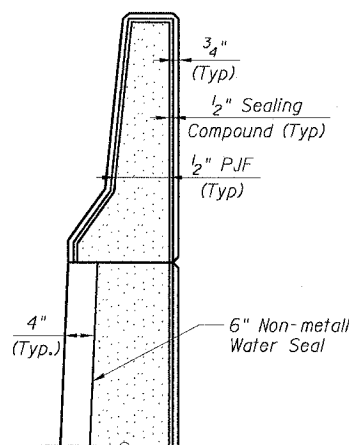
EXPANSION JOINT
