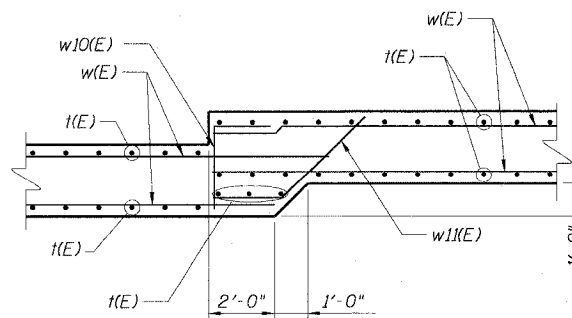
DETAIL 3
