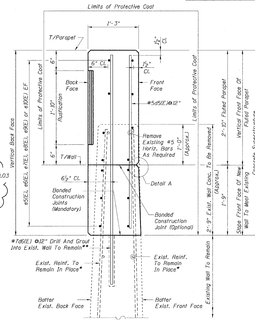
SECTION K-K
