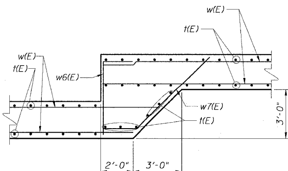
DETAIL 1
