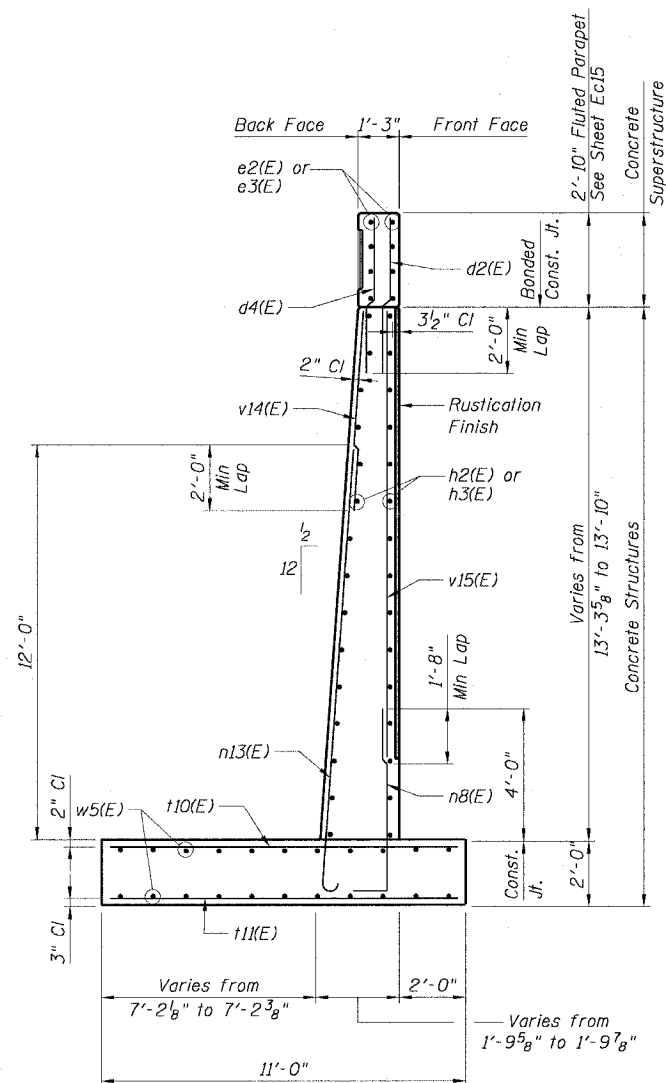
SECTION I-I
