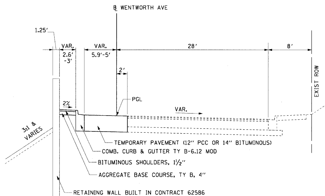
TEMPORARY PAVEMENT DETAIL STA 131+44.62 TO STA 131+93.21
