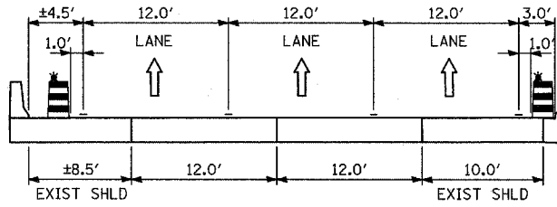
SECTION O-O
