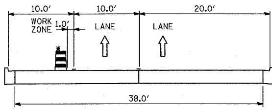
SECTION M-M
