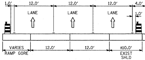
SECTION N-N
