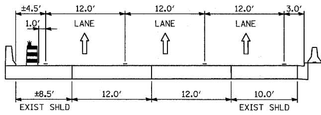
SECTION P-P
