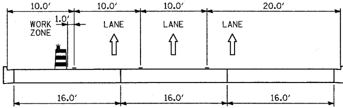
SECTION L-L
