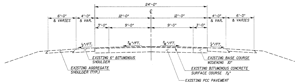
EXISTING ROADWAY TYPICAL SECTION
