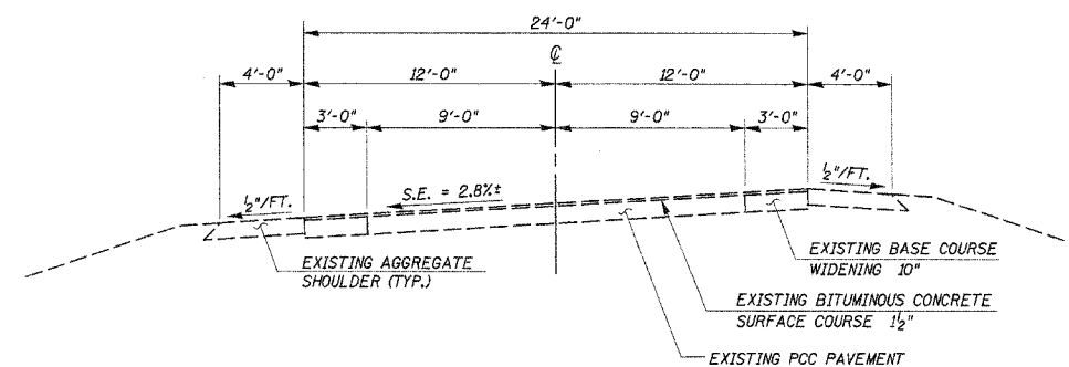
EXISTING ROADWAY TYPICAL SECTION
