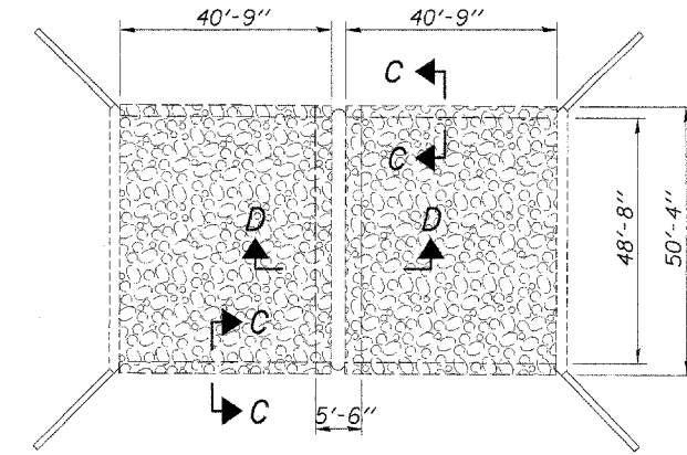
SLOPE MATTRESS LOCATION PLAN* (Existing)
