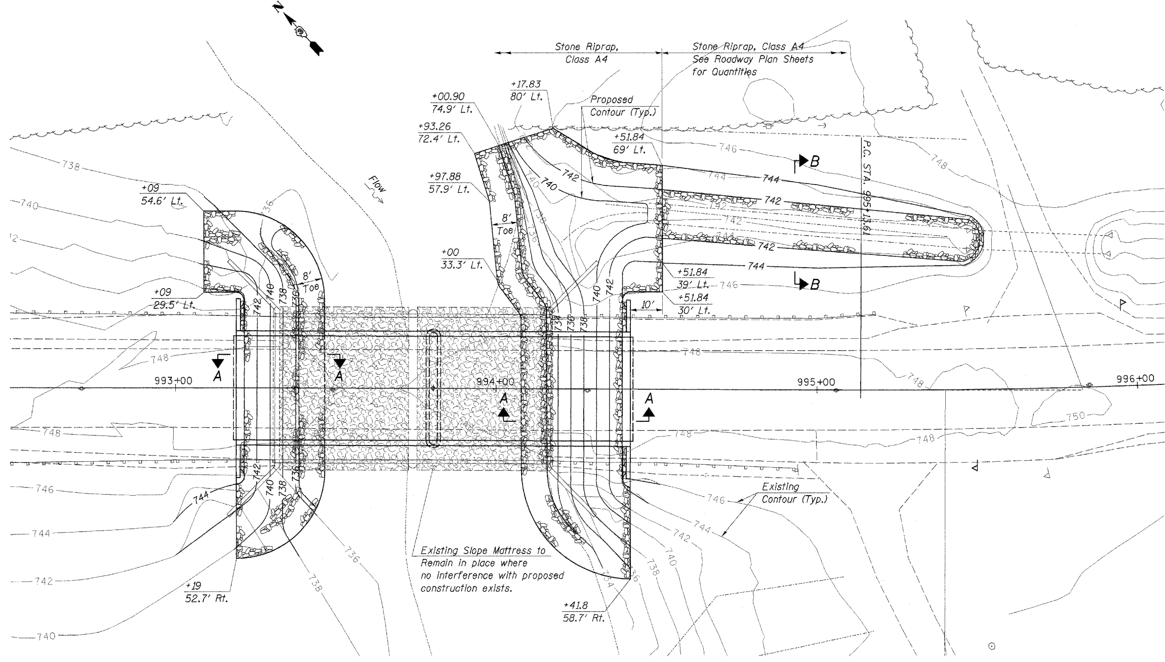
PLAN
