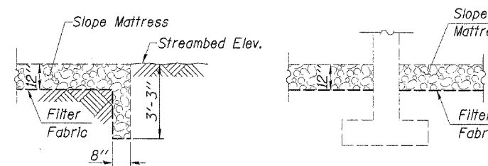
SECTION C-C* Existing Toewall
