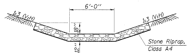
SECTION B-B STONE RIPRAP DITCH
