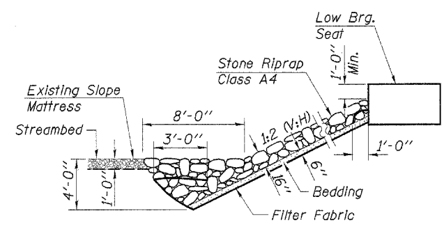
SECTION A-A STONE RIPRAP ANCHOR DETAIL
