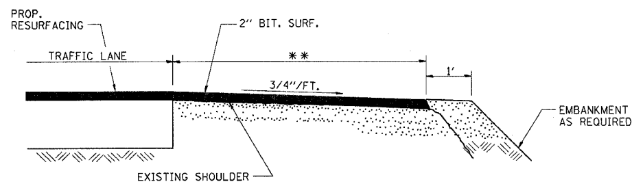
SECTION A-A MAILBOX TURNOUT DETAILS
