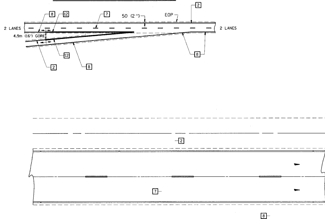
TYPICAL ENTRANCE RAMP TERMINAL
