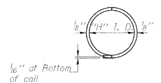
PLAN-COIL WIRE
