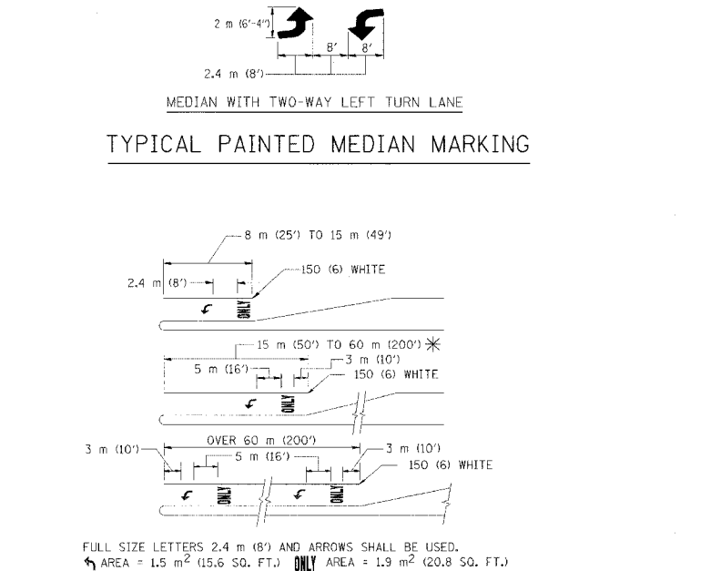
TYPICAL LEFT (OR RIGHT) TURN LANE
