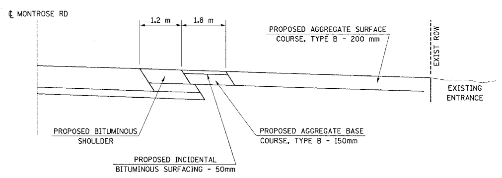
SECTION THROUGH PRIVATE ENTRANCE
