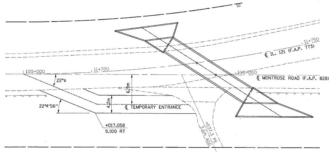
DETAIL OF TEMPORARY ENTRANCE
