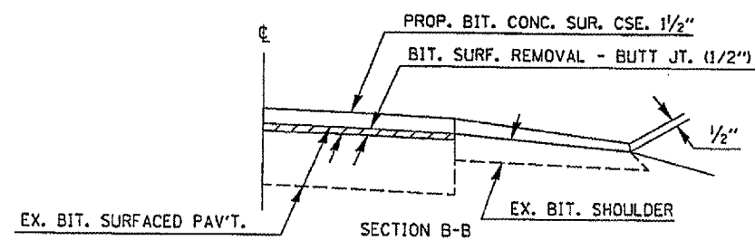
SECTION B-B NOT TO SCALE
