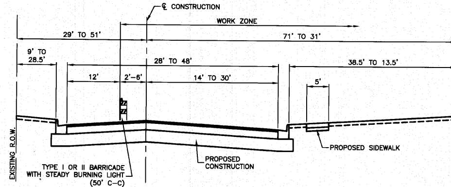
TYPICAL CROSS SECTION STAGE 2 - 175TH STREET STA 50+94.84 TO STA 56+17.70
