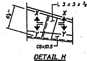
DETAIL H
