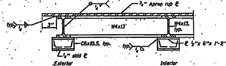
SECTION V-V (8 locations)
