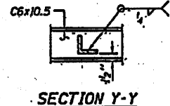
SECTION Y-Y
