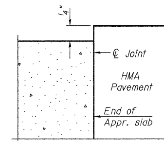
FLEXIBLE PAVEMENT
