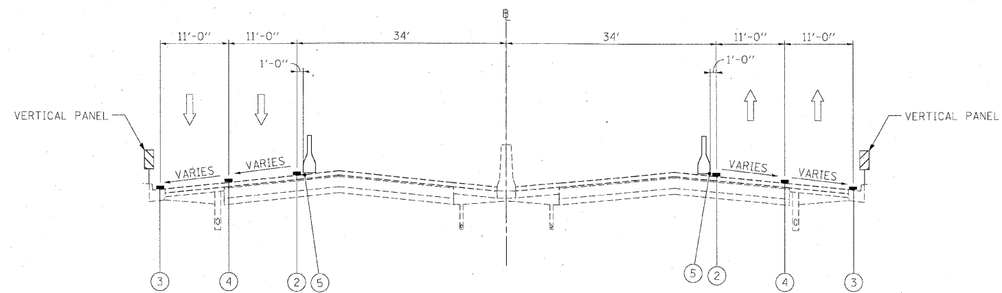
WESTBOUND MAINTENANCE OF TRAFFIC EASTBOUND TYPICAL SECTION STAGE 2 STA 503+43 TO 530+10 BRIDGE OMISSION STA 505+97 TO 526+15 STA 506+97 TO STA 509+30 STA 524+98 TO STA 525+90
