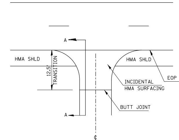
SIDEROAD DETAIL
