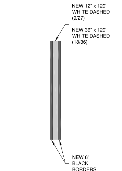
4 RUNWAY 18/36 AND 9/27 CENTERLINE DASHED N.T.S.
