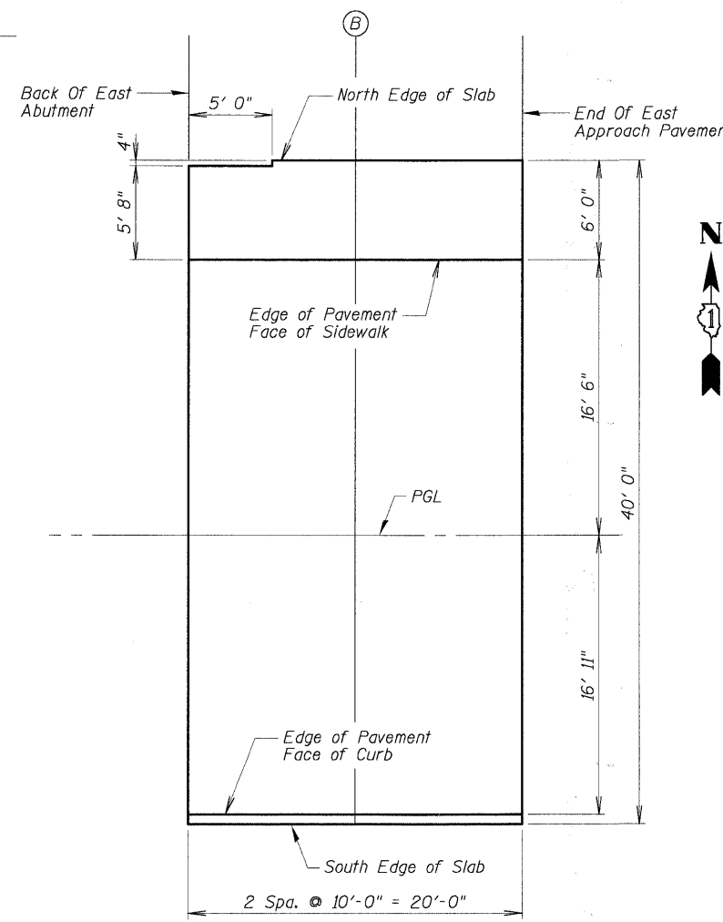
EAST APPROACH PAVEMENT
