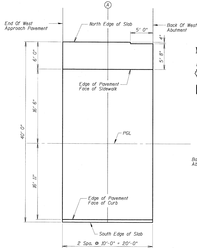
WEST APPROACH PAVEMENT
