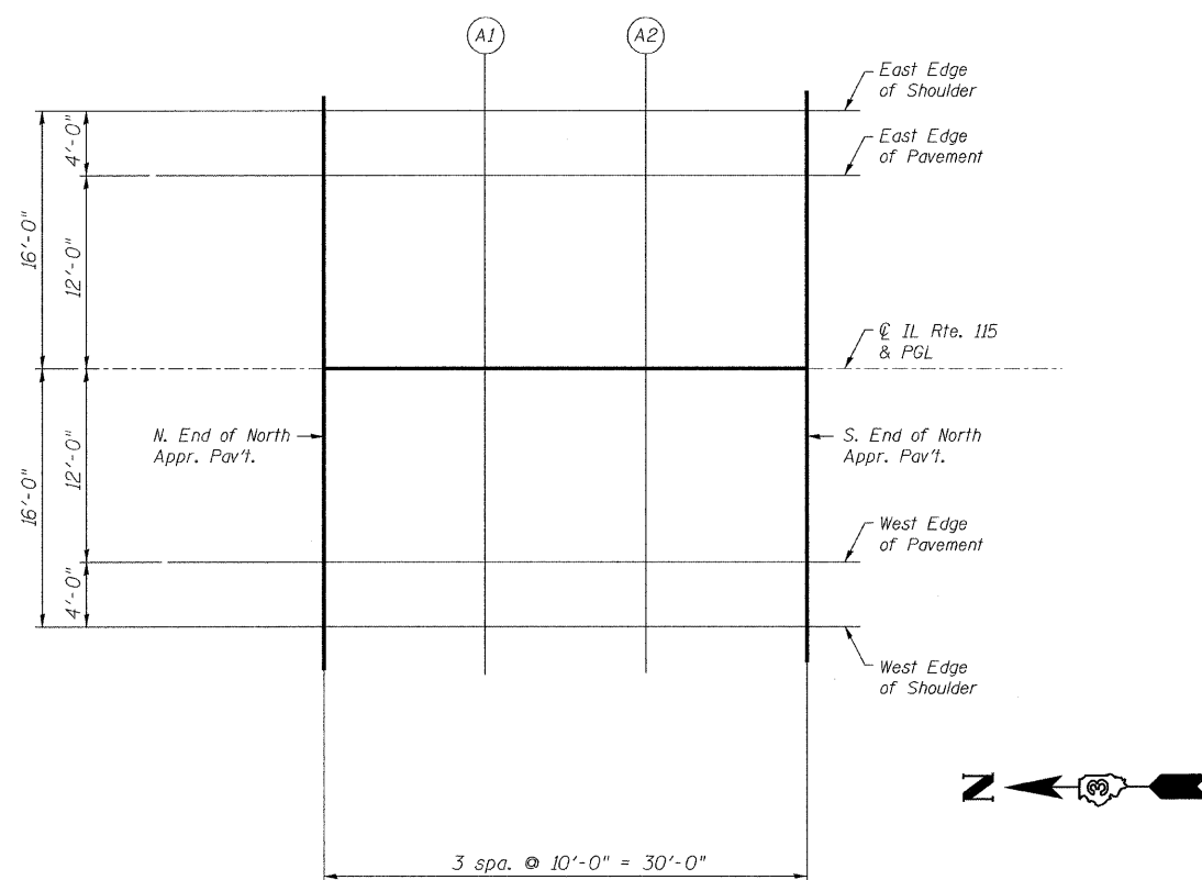
NORTH APPROACH SLAB
