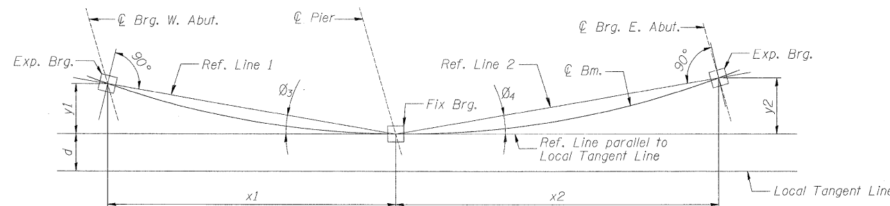
BEARING ORIENTATION
