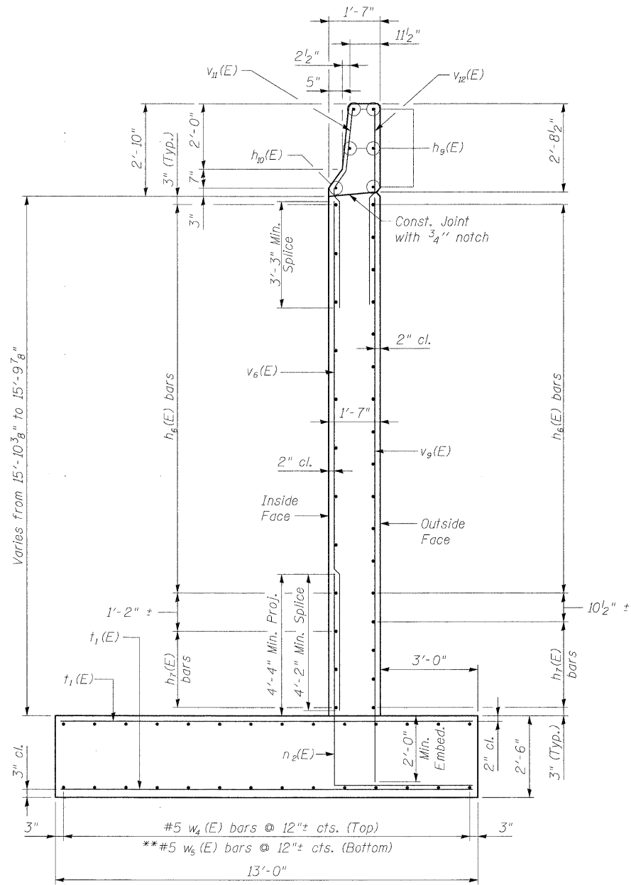
SECTION B-B
