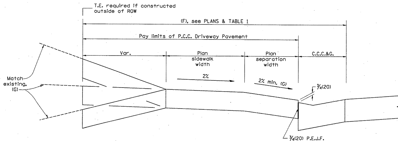
SECTION B-B
