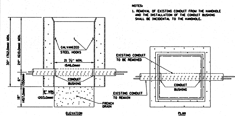
DETAIL HANDHOLE TO INTERCEPT EXISTING CONDUIT
