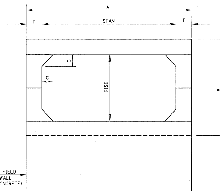
END VIEW
