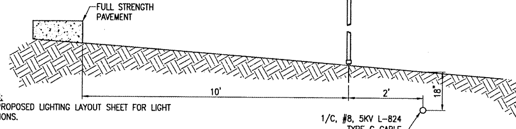
PROFILE VIEW
