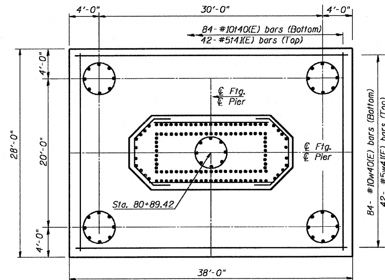
FOOTING PLAN
