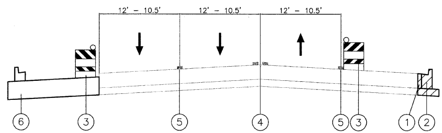
TYPICAL SECTION - TEMPORARY LANE CLOSURE (SEE MOT NOTES FOR PERMITTED HOURS)
