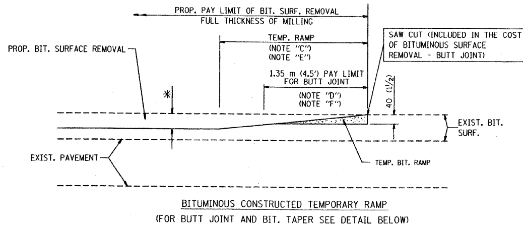
OPTION 2 TYPICAL TEMPORARY RAMP
