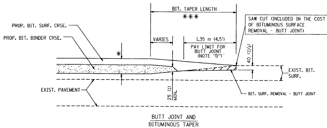
TYPICAL BUTT JOINT AND BITUMINOUS TAPER FOR MILLING AND RESURFACING
