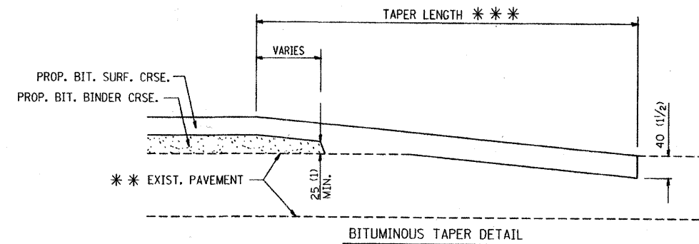
TYPICAL BUTT JOINT AND BITUMINOUS TAPER FOR RESURFACING ONLY
