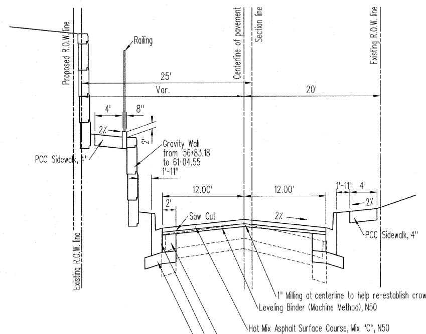
Proposed Typical Cross Section #2 Station 56+59.44 to Station 63+26.71 Tyler Avenue to Harrison Avenue
