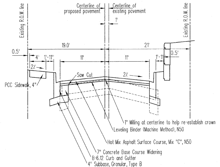
Proposed Typical Cross Section #5 Station 70+26.03 to Station 73+50.00 Van Buren Avenue to Jackson Avenue
