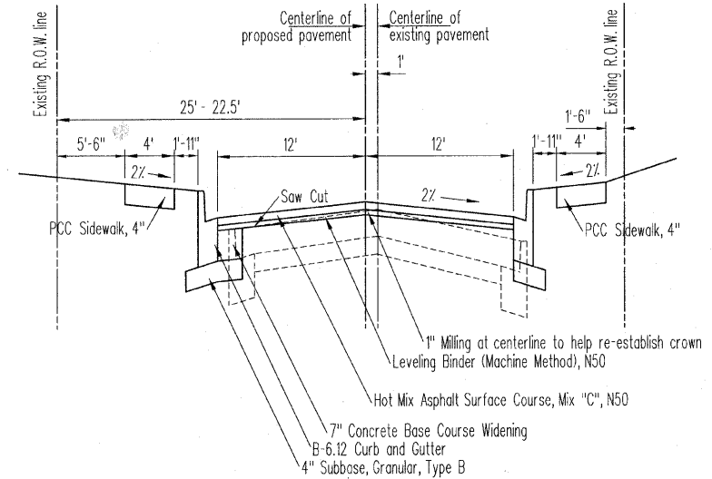
Proposed Typical Cross Section #4 Station 66+54.68 to Station 70+26.03 Town Branch to Van Buren Avenue
