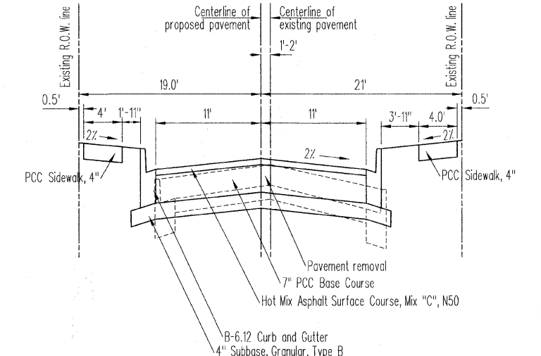
Proposed Typical Cross Section #6 Station 73+50.00 to Station 78+20.00 Jackson Avenue to Madison Avenue
