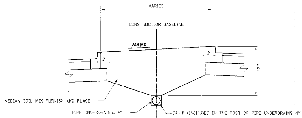
LANDSCAPE MEDIAN DETAIL - STA. 46+74 TO STA. 48+49 NOT TO SCALE
