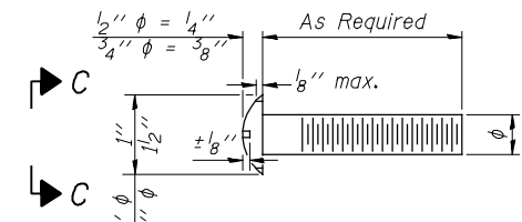
DETAIL OF 1/2 inch & 3/4 inch ROUND HEAD BOLTS
