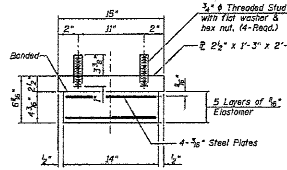
BEARING ASSEMBLY
