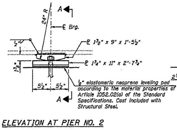
FIXED BEARING (At Pier No. 2 - 6 Required)
