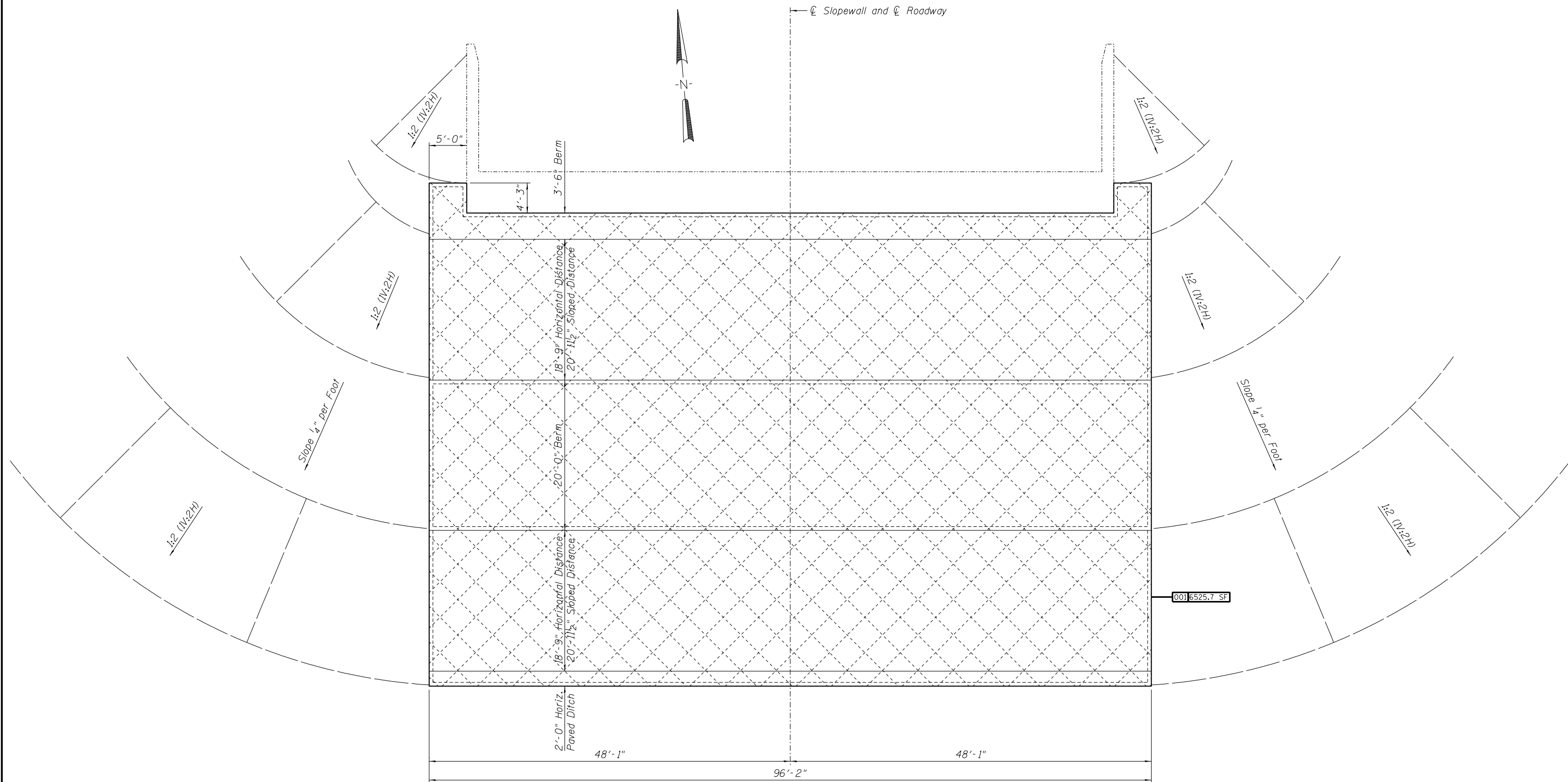
SLOPEWALL PLAN
