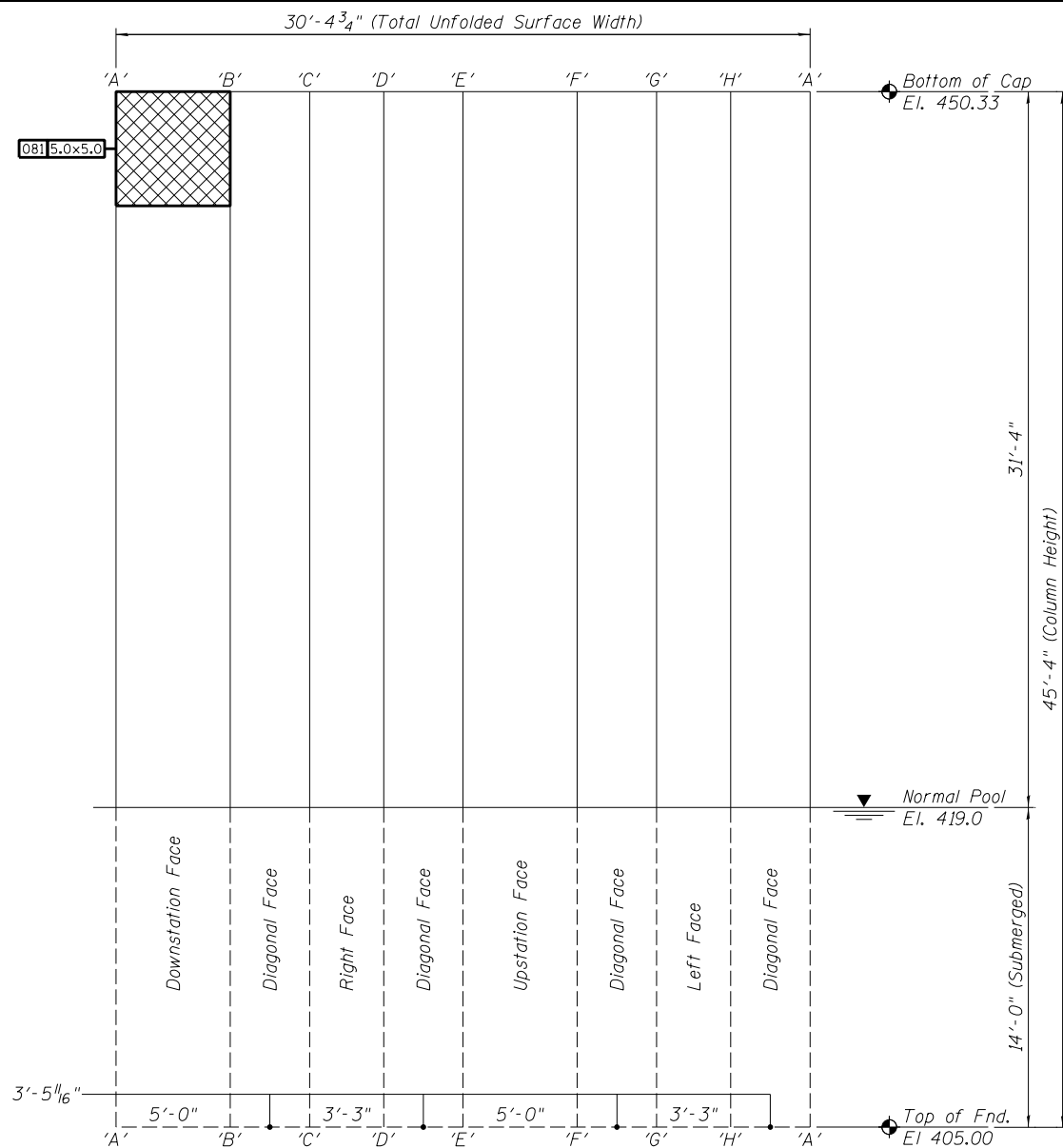
PIER NO. 4 - ELEVATION - LEFT COLUMN Column Surface Shown Unfolded
