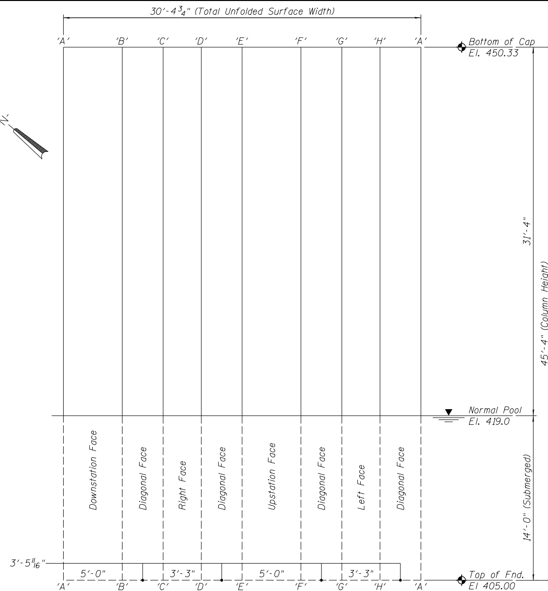
PIER NO. 4 - ELEVATION - RIGHT COLUMN Column Surface Shown Unfolded
