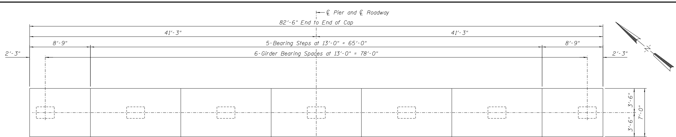
PIER CAP - PLAN - PIER 14
