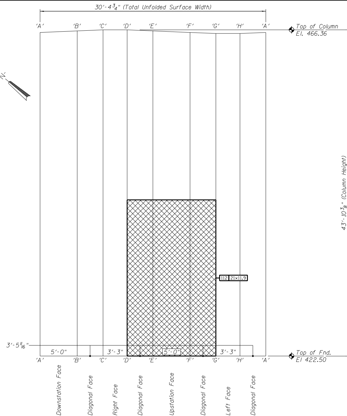
PIER NO. 14 - ELEVATION - RIGHT COLUMN Column Surface Shown Unfolded
