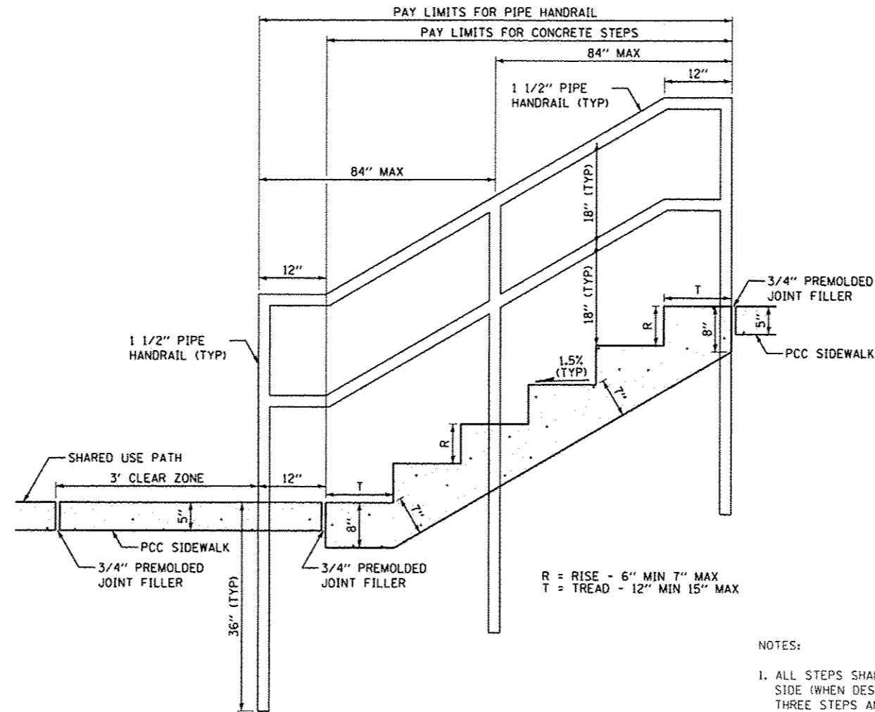
TYPICAL STEP AND HANDRAIL DETAIL
