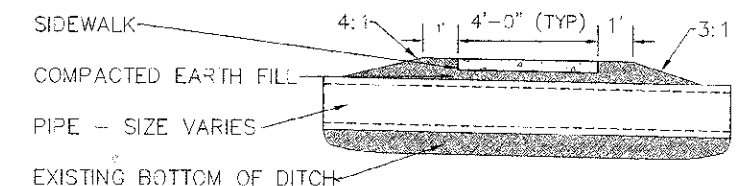
PIPE CULVERT, CLASS C, TYPE 1 SECTION A-A NOT TO SCALE
