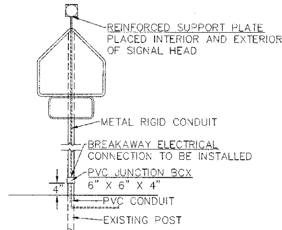
POST MOUNTED FLASHING BEACON NOT TO SCALE
