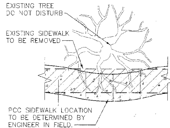
TYPICAL TREE TRANSITION NOT TO SCALE
