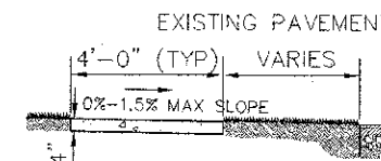
TYPICAL SIDEWALK SECTION NOT TO SCALE
