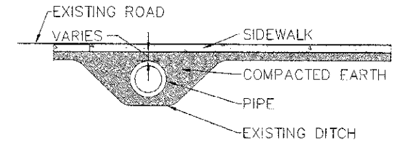
SIDEWALK OVER PIPE CULVERT PLAN B-B NOT TO SCALE
