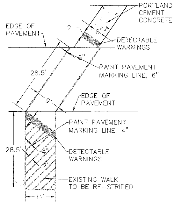
SCHOOL CROSSING PAINT DETAIL NOT TO SCALE
