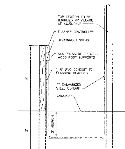
SERVICE INSTALLATION, TYPE A (MODIFIED)
