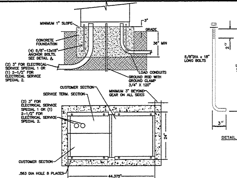
PEDESTAL/ENCLOSURE BASE DETAIL NO SCALE
