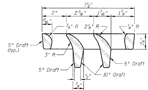
VANE GRATE DETAIL
