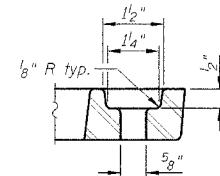
BOLT HOLE DETAIL
