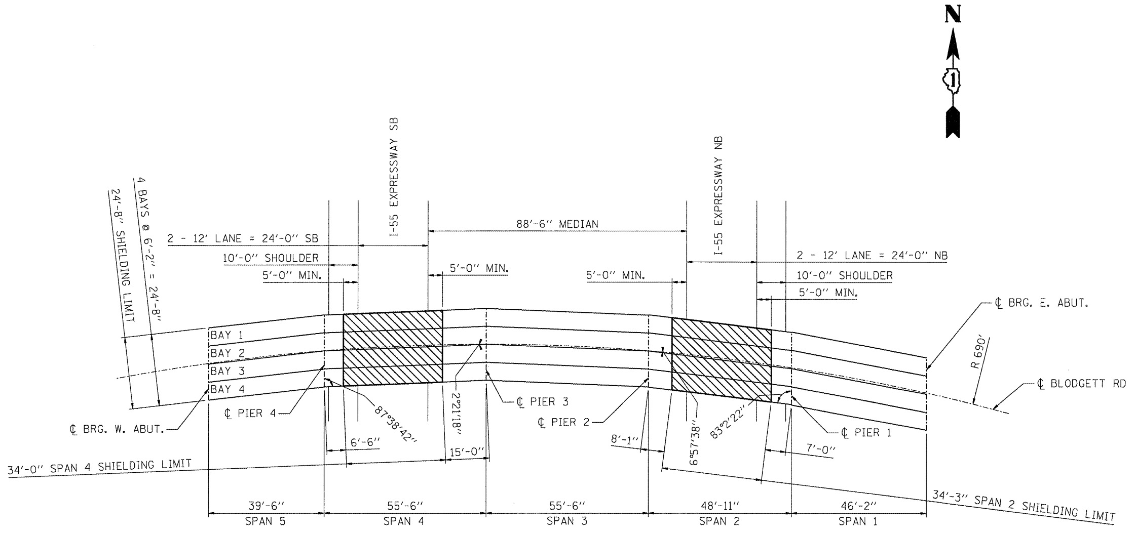
FRAMING PLAN
