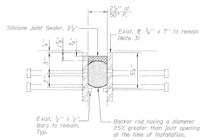
SECTION B-B (At East Abutment)
