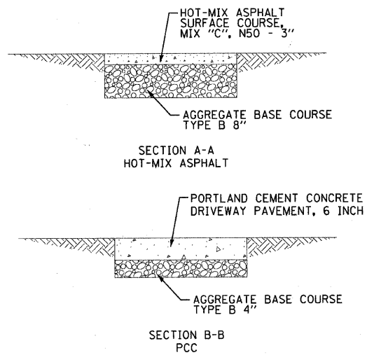
DRIVEWAY DETAIL NO SCALE
