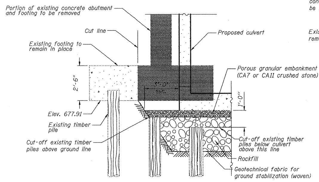
SECTION J-J
