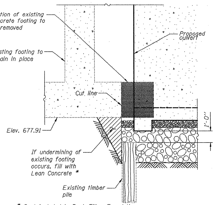
SECTION K-K
