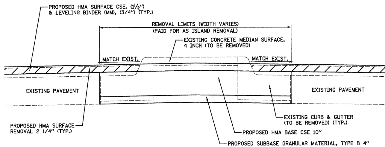
DETAIL FOR ISLAND REMOVAL
