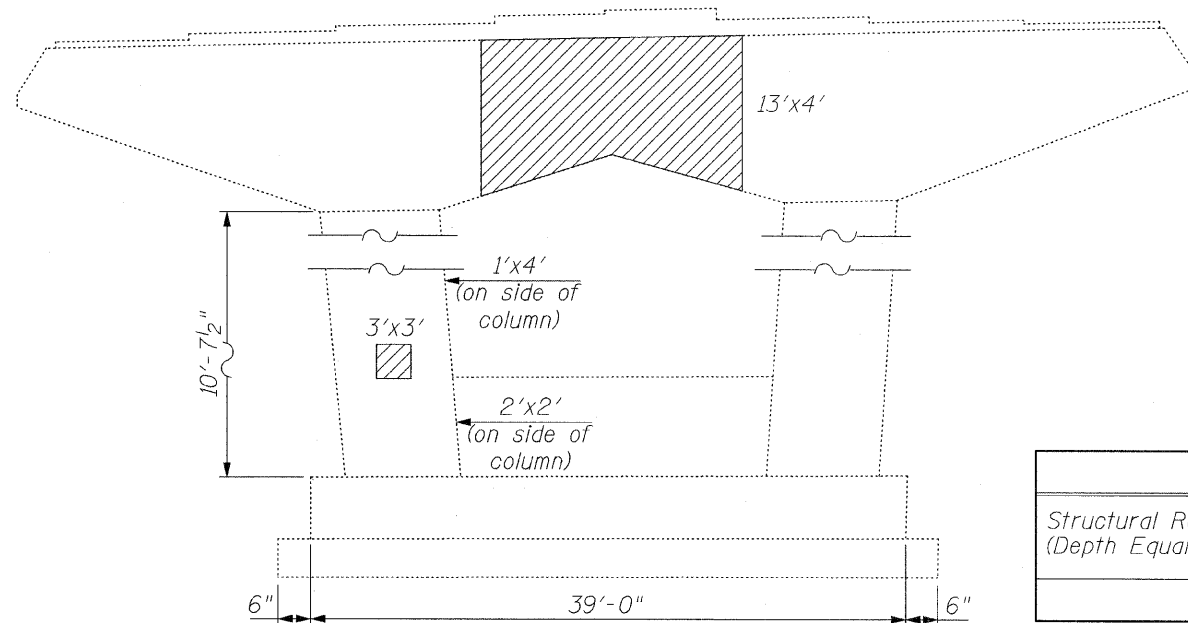
NORTH FACE (Looking South)
