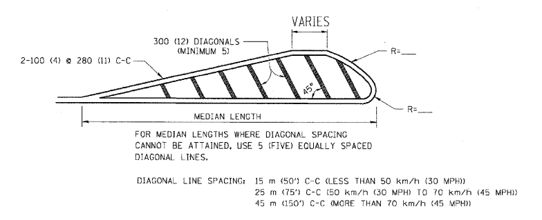
TYPICAL PAINTED MEDIAN MARKING
